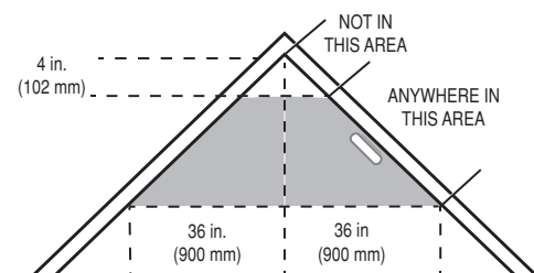
Figure 8. Example of proper mounting for Detectors with peaked ceilings
