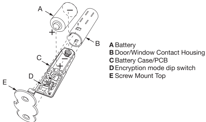
Figure 3 Battery Compartment and Polarity
